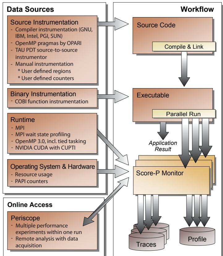
Score-P workflow and performance data sources
